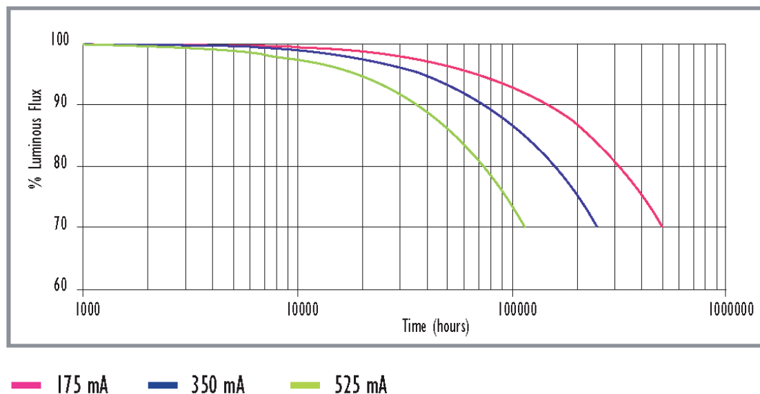
Graph showing typical lumen depreciation with drive current and time
